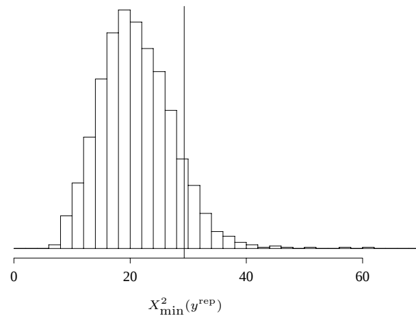
Figure 6. Histogram of 1000 simulations from the reference distribution for X^2_{\min}(y^{\text{rep}}) , the minimum \chi^2 statistic for the mortality rates, using the posterior predictive distribution. The vertical line represents X^2_{\min}(y) , the observed value of the minimum \chi^2 statistic.
